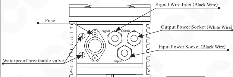
SDVC21-LP (10A)
